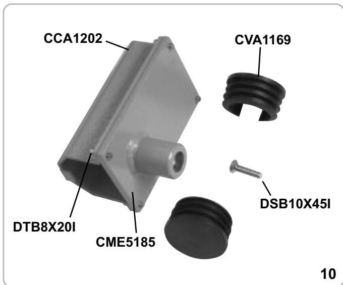
Fixing hub for \varnothing 80 mm boom arm. code ACG8548
